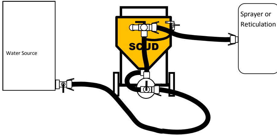
SCUD 150 Mixer typical set up
